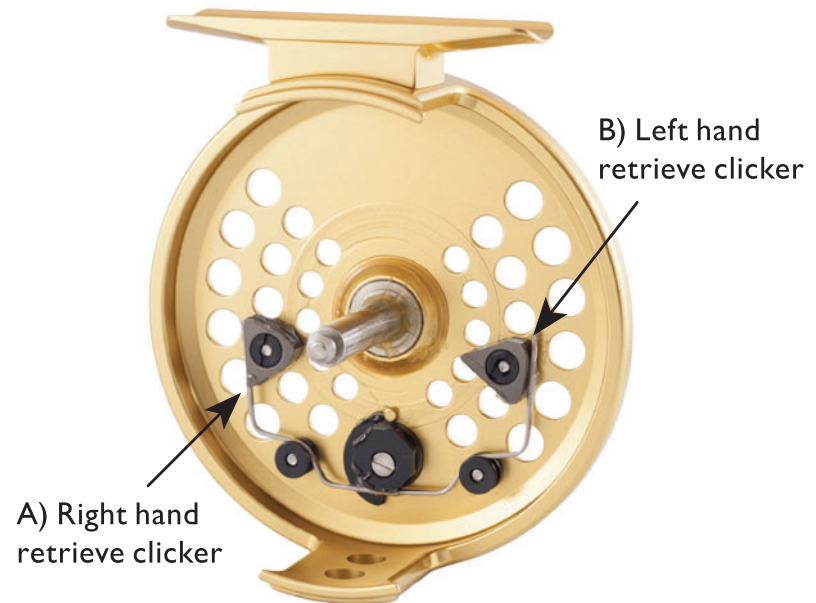
Figure 2 – Left-hand retrieve setup
