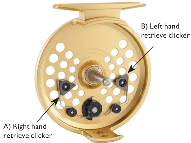
Figure 1 – Right-hand retrieve setup
