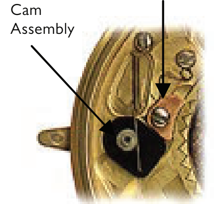
Pawl Assembly
